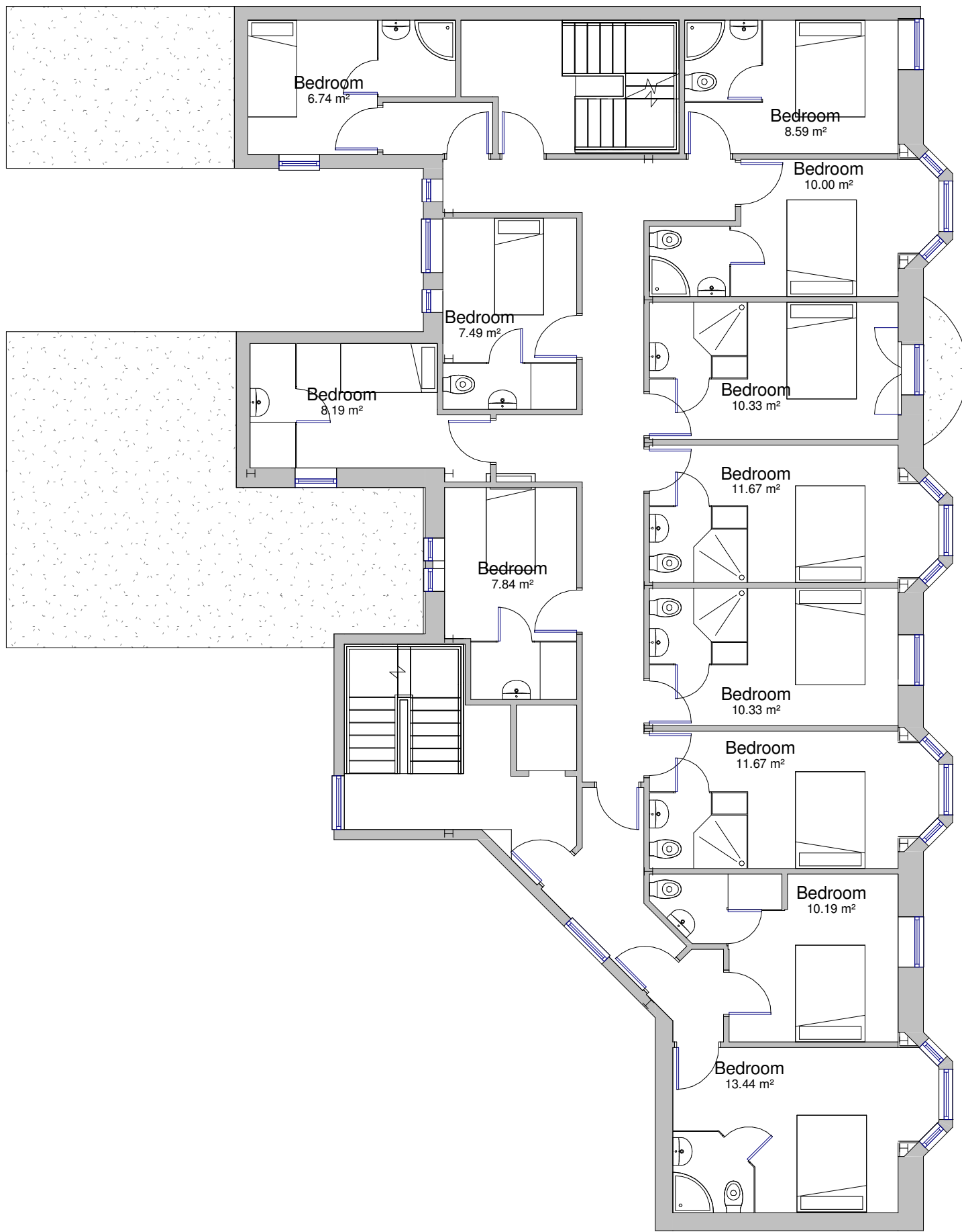
First Floor Proposed 1 : 100
